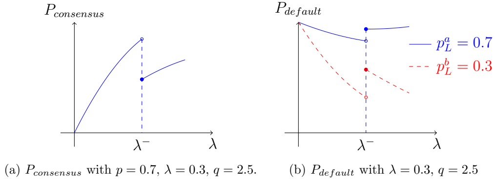
Figure 4: The effect of \lambda on the first two indicators of polarization.
